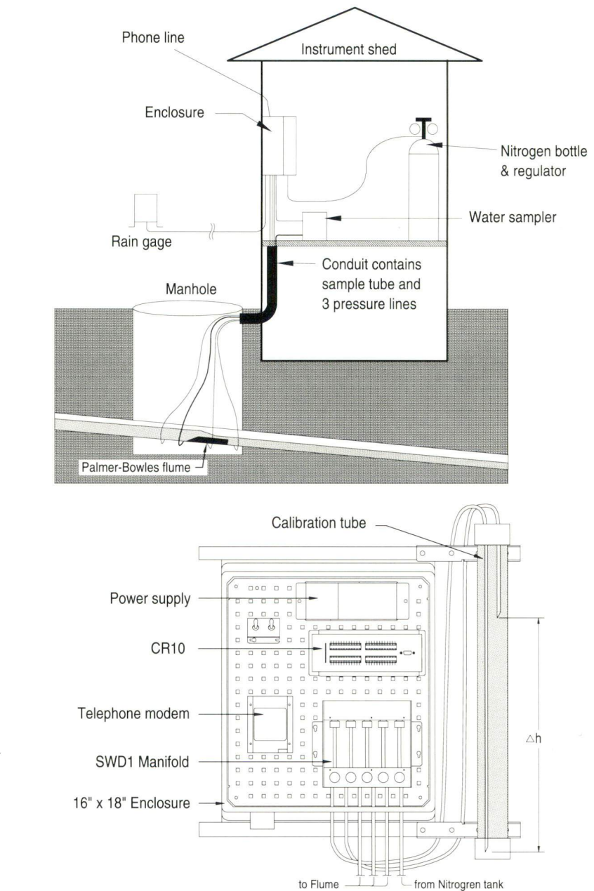
Figure 1. Typical installation (above); SWD1 components (below).
