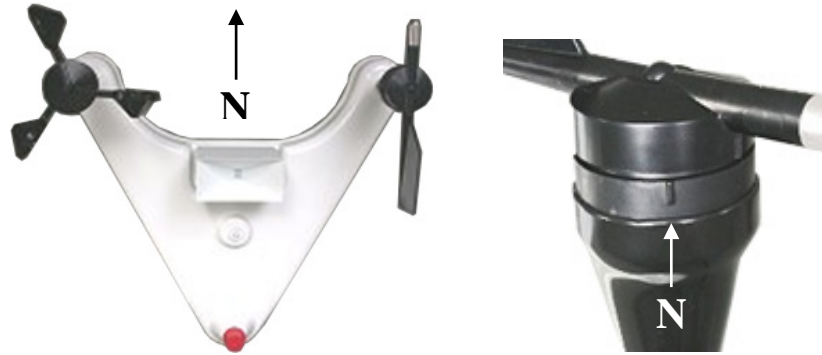
FIGURE 5-9. Accurate wind direction measurements require the reference line on the wind direction sensor (right) to be aligned with Magnetic North
