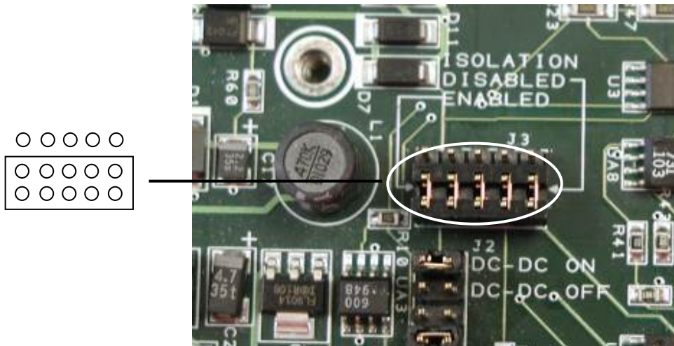
FIGURE 2-3. SDM-CAN Isolation disabled
