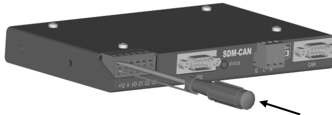
FIGURE 2-5. Using the Spring Loaded Terminal Blocks (Front Option)
