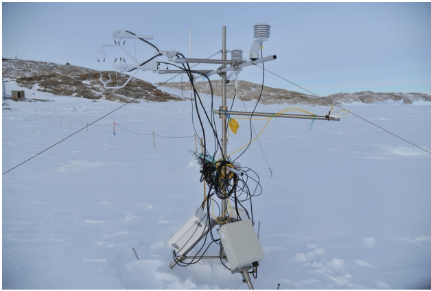
Figure 2. The eddy-covariance station located in the coastal landfast sea ice area of Antarctica Zhongshan Station ( 69^{\circ}22' S , 76^{\circ}22' E ). It was configured with the IRGASON integrated CO_2/H_2O open-path gas analyzer and three-dimensional sonic anemometer, CNR4 four-component net radiometer, HMP155A air temperature and relative humidity probe, and SI-111 infrared radiometer.
