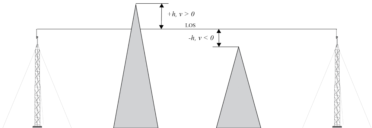
FIGURE 5-1. Diffraction Parameter
