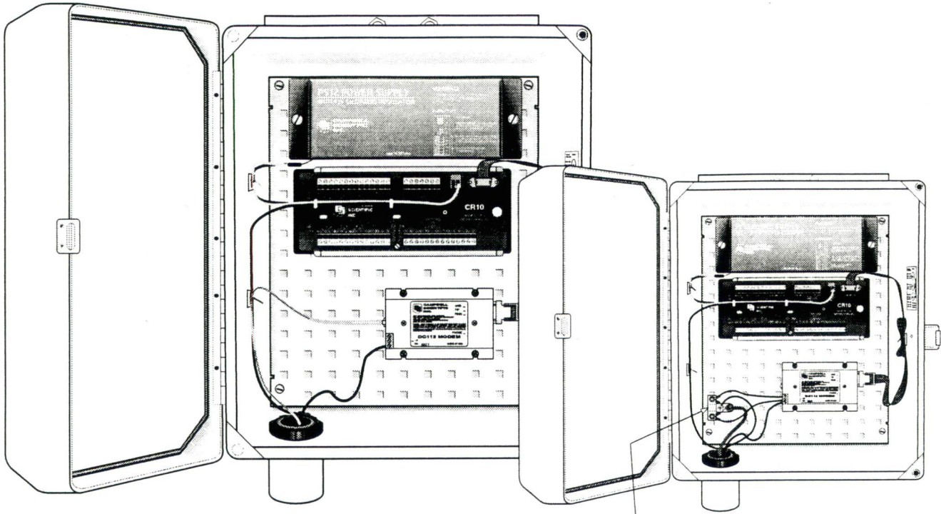
DC112 in ENC 12/14 enclosure with CR10X datalogger and PS12 power supply. In this example, the phone company has installed a surge protector below the field of view.
