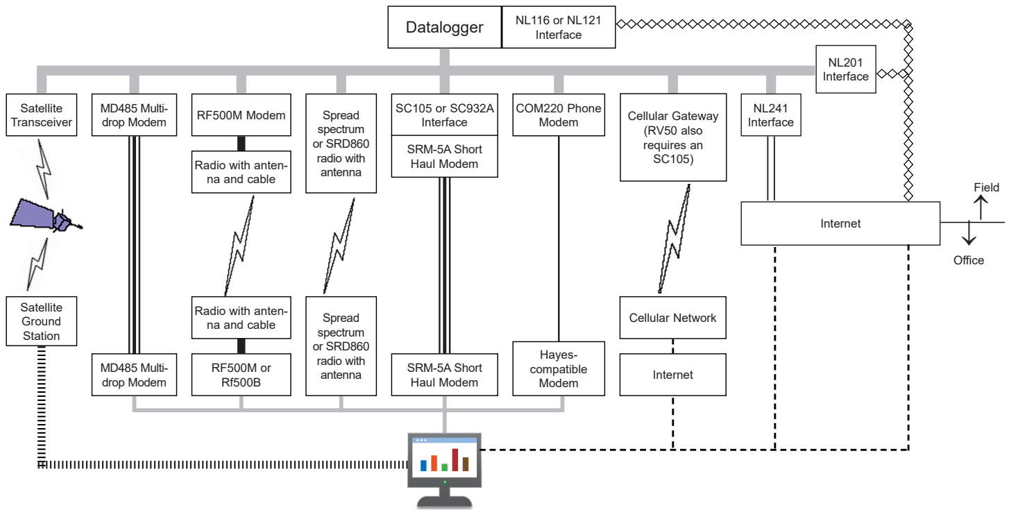
Laptop or desktop computer running Datalogger Support Software (see the Software Support section on pg 5)
