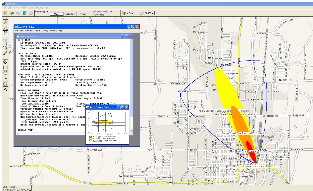
Figure 5 - ALOHA® Plume
