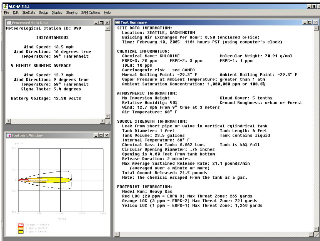
Figure 4 - CAMEO®/ALOHA® Screen
