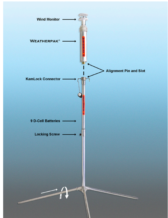
Figure 1 – Assembly
