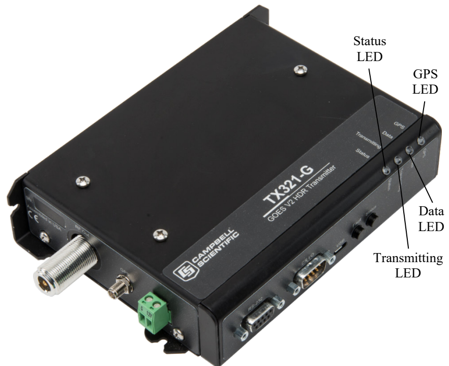
FIGURE 7-1. TX321 LEDs
