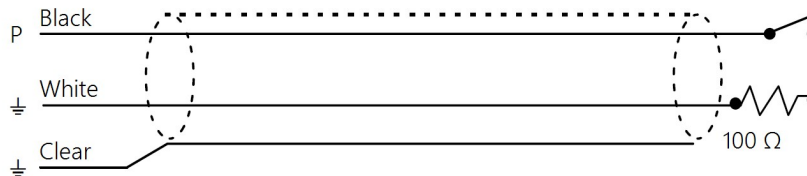
FIGURE 8-1. TE525-series rain gage schematic
