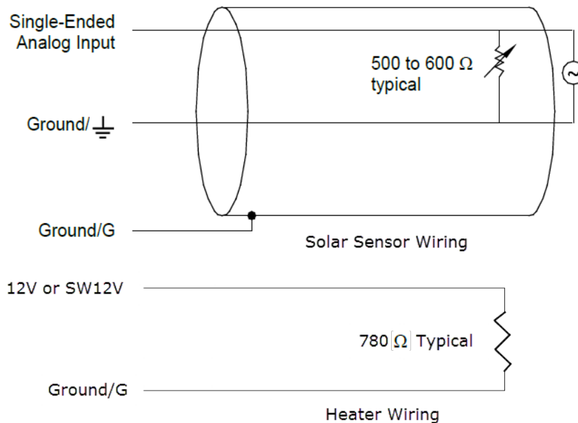
FIGURE 7-1. Schematic diagram
