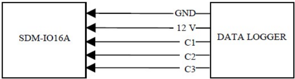
(a) Connection with data logger supply
