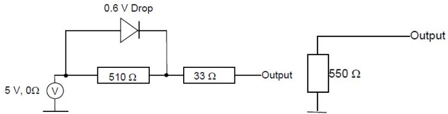
(b) Output set ON
