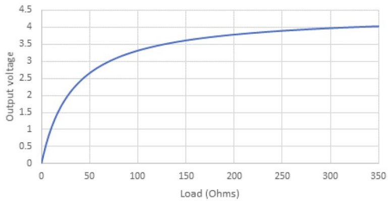
(e) Output voltage versus resistive load
