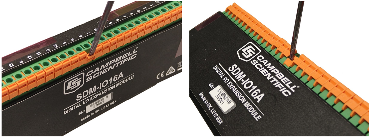
FIGURE 3-2. Use of terminal blocks
