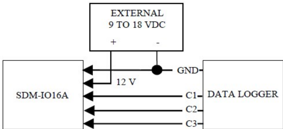
(b) Connection with external supply
