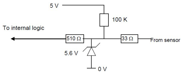
(a) Input biasing and protection
