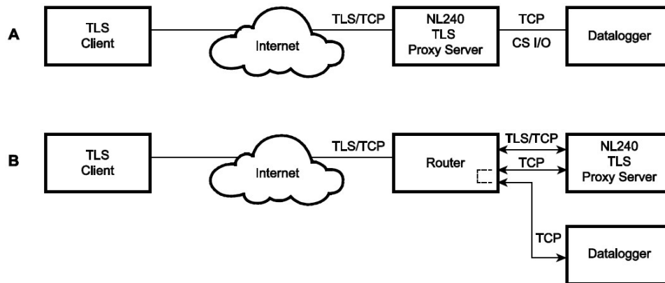
FIGURE 8-4. TLS proxy server configurations
