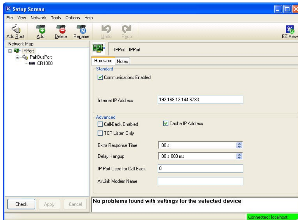
FIGURE 8-3. CS I/O serial server LoggerNet setup
