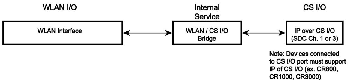
FIGURE 4-2. Bridge mode enabled
