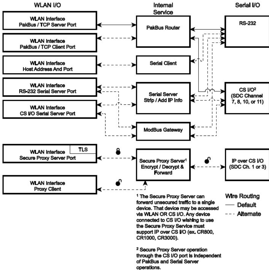
FIGURE 4-3. Bridge mode disabled
