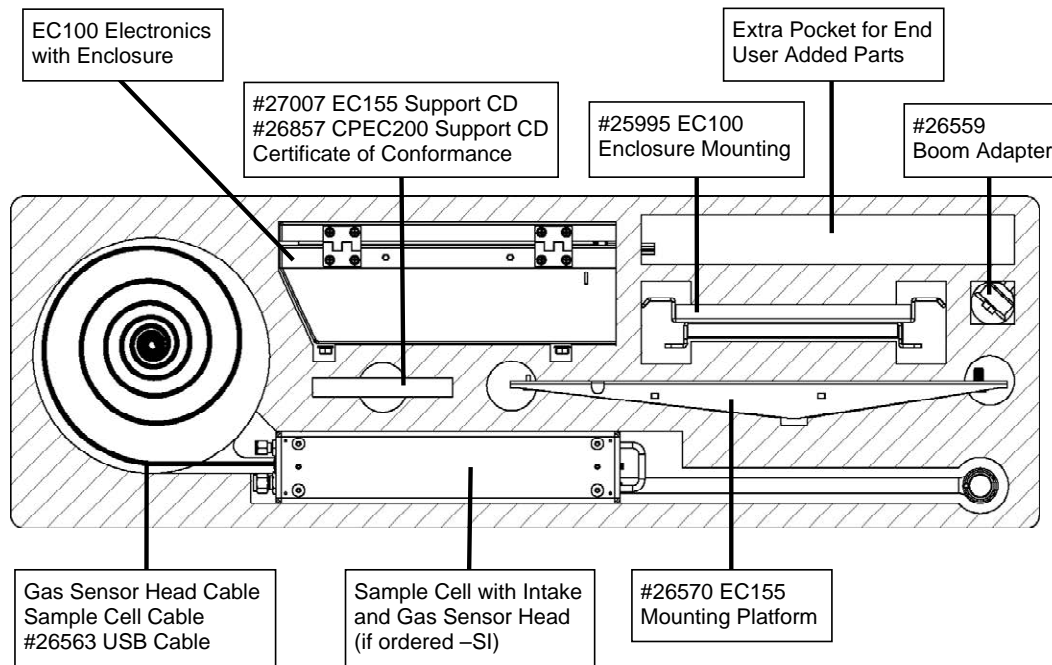
FIGURE 1. CPEC200 with Sample Cell Option -SI
